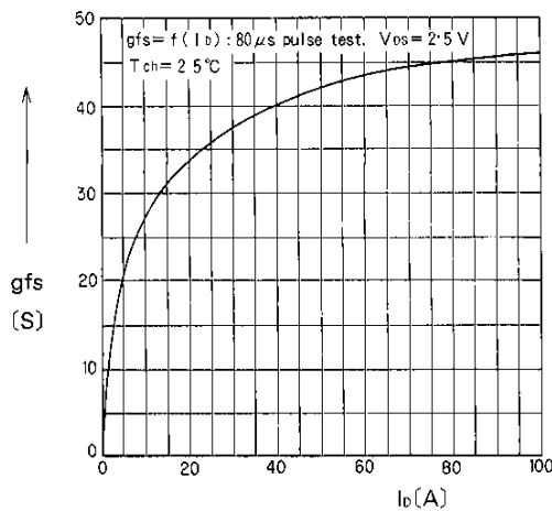
Typical Forward Transconductance
