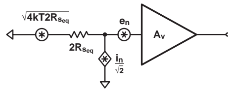
Figure 4: Noise Model with R_f || R_g = R_{seq}
