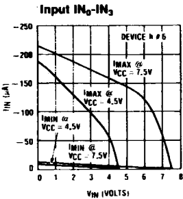
Figure 7 : ETL9320/L9321/L9322 Input/Output Characteristics.
