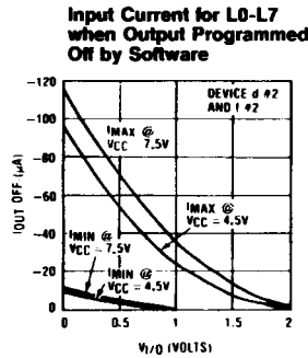
Figure 7 : ETL9320/L9321/L9322 Input/Output Characteristics.
