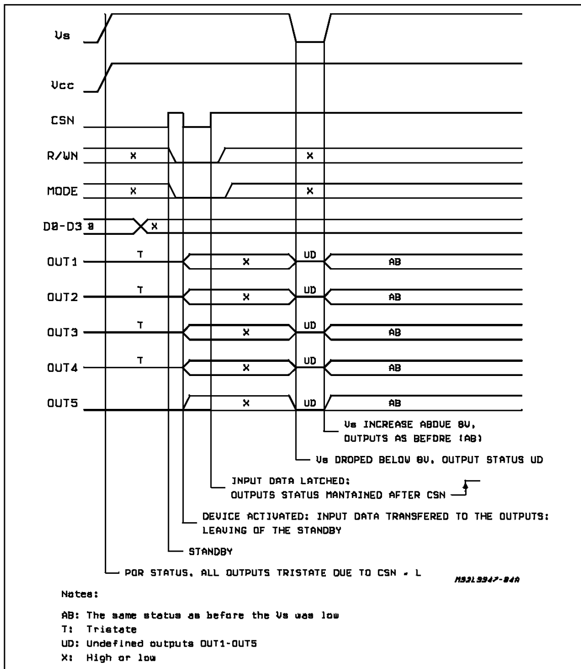
Figure 2: System Startup Sequence
