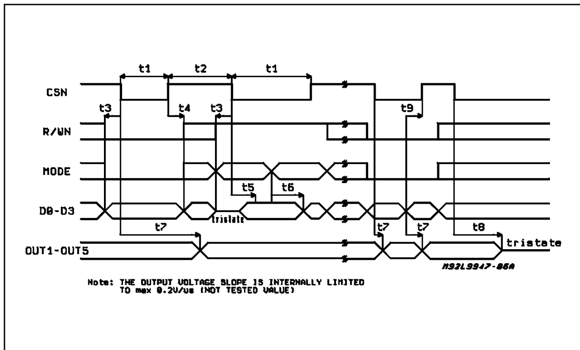
Figure 4: Bus and Outputs Timing Diagram
