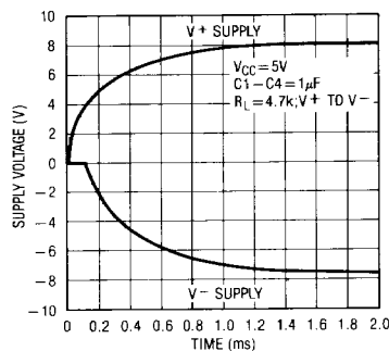
Supply Generation from V_{\text{CC}} or Shutdown
