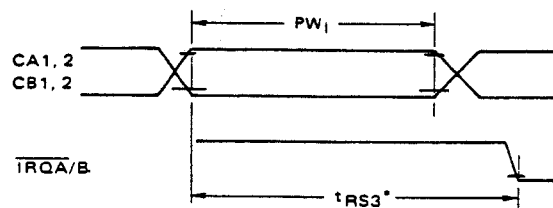
FIGURE 13 — INTERRUPT PULSE WIDTH AND \overline{\text{IRQ}}/\text{B} RESPONSE
