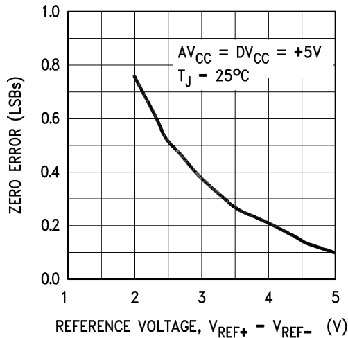
Zero (Offset) Error vs. Reference Voltage
