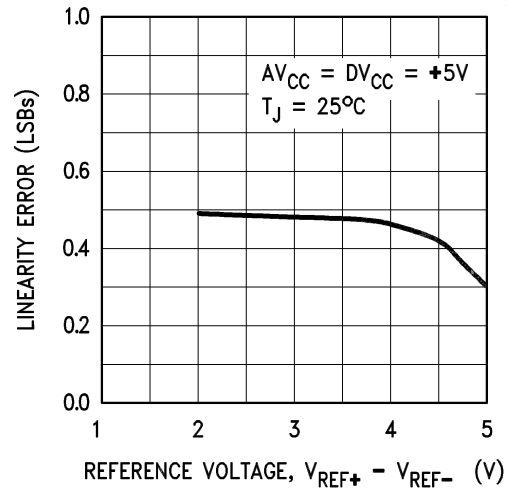
Linearity Error vs. Reference Voltage
