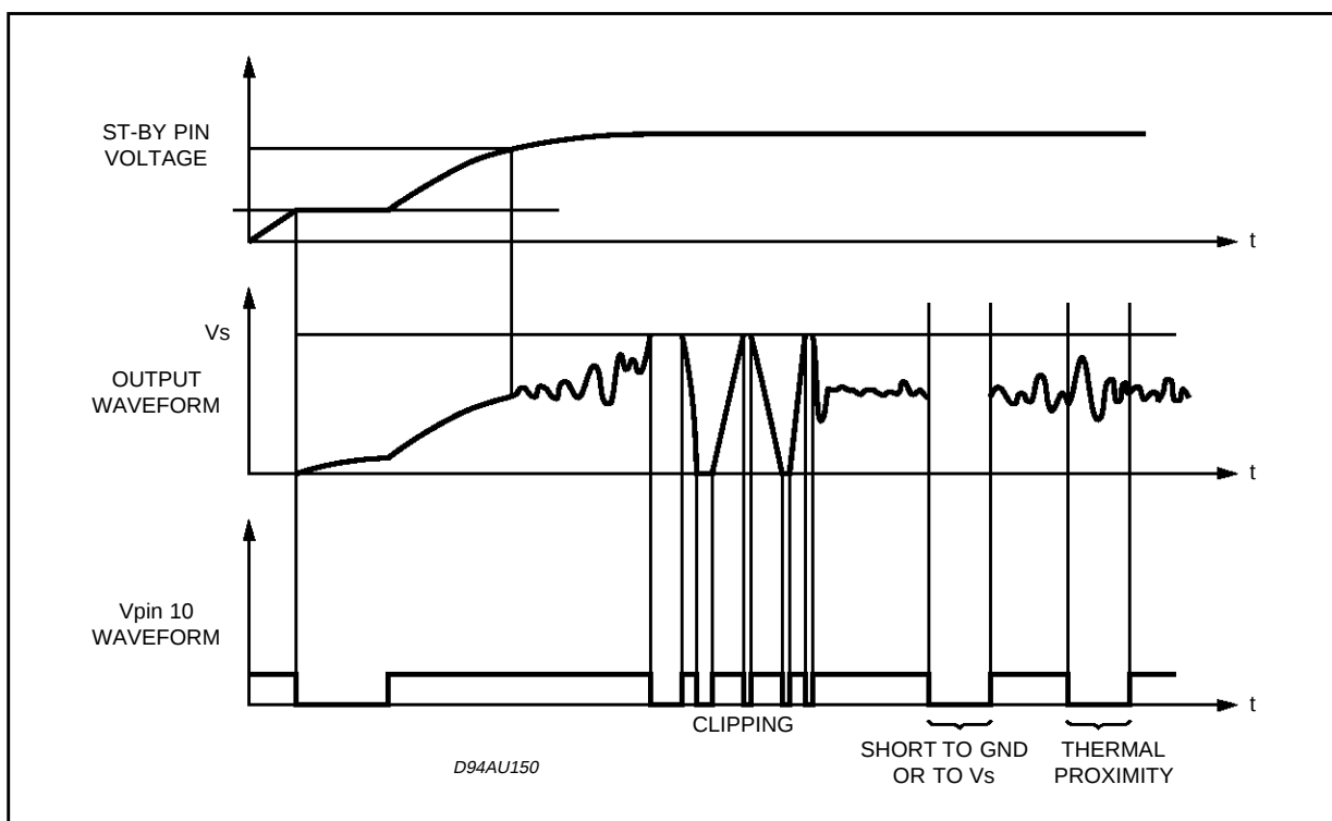
Figure 25: Waveforms
