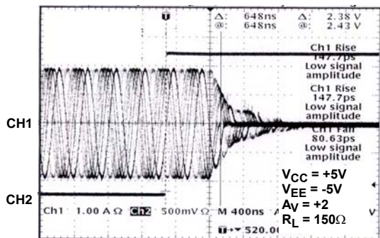
FIGURE 15. TURN OFF DELAY
