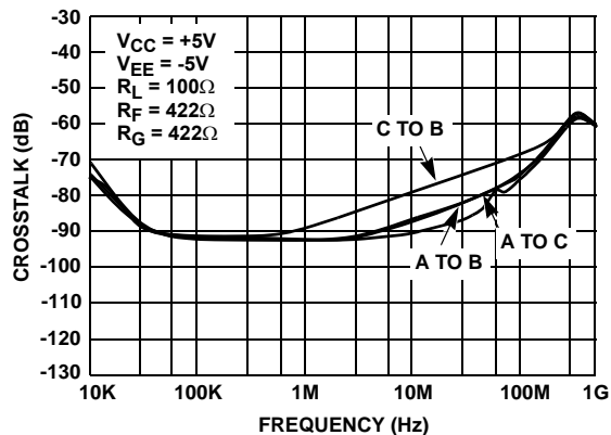
FIGURE 18. CHANNEL CROSSTALK BETWEEN CHANNELS
