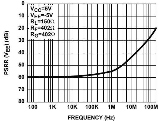
FIGURE 12. PSRR -5V
