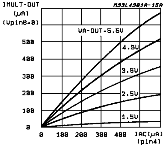
Figure 1: MULTI-OUT vs. I_{AC} ( V_{RMS} = 1.7V ; V_{LFFD} = 5.1V )
