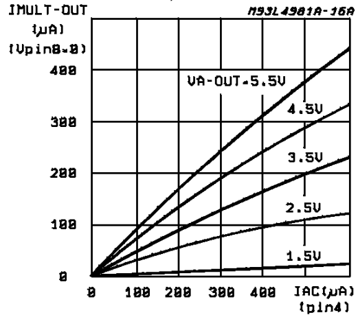
Figure 2: MULTI-OUT vs. I_{AC} ( V_{RMS} = 2.2V ; V_{LFFD} = 5.1V )
