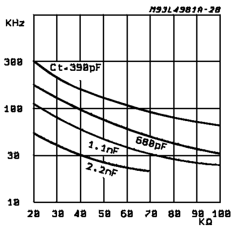
Figure 18: Oscillator Diagram
