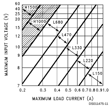
FIGURE 4. LM2575(HV)-5.0
