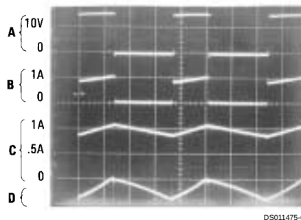
Switching Waveforms
