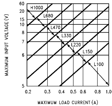
FIGURE 3. LM2575(HV)-3.3
