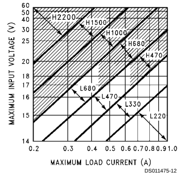
FIGURE 5. LM2575(HV)-12
