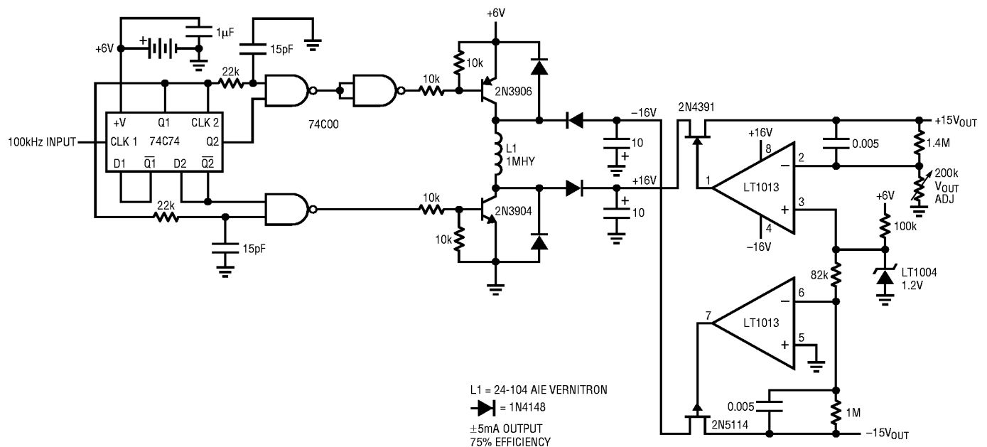
6V to \pm 15V Regulating Converter
