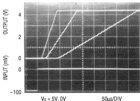
V_S = 5V, 0V 50 \mu s /DIV
