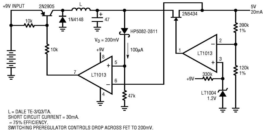
Low Power 9V to 5V Converter
