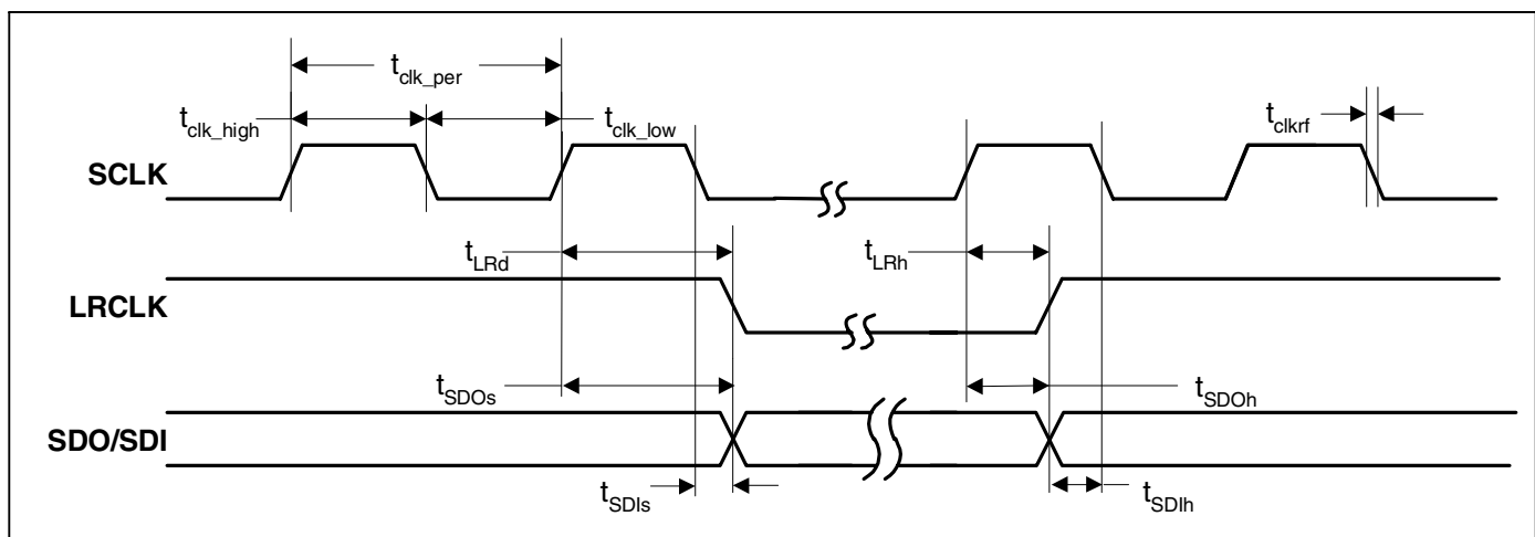
Figure 18. Inter-IC Sound (I 2 S) Timing Measurement
