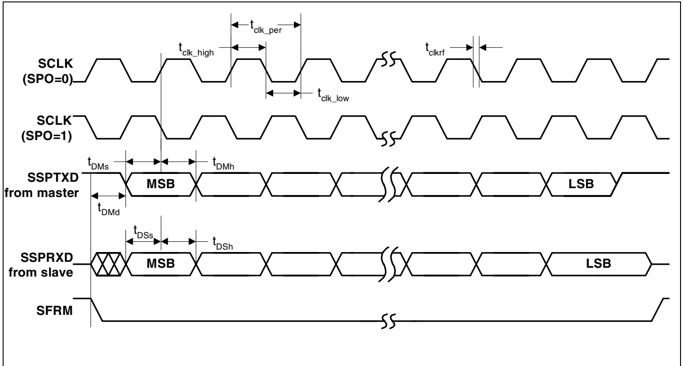
Figure 17. SPI Format with SPH=1 Timing Measurement
