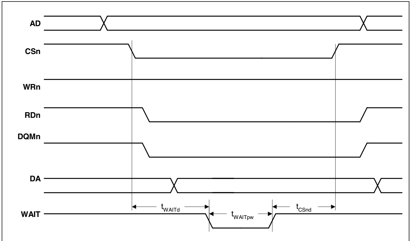
Figure 11. Static Memory Single Read Wait Cycle Timing Measurement
