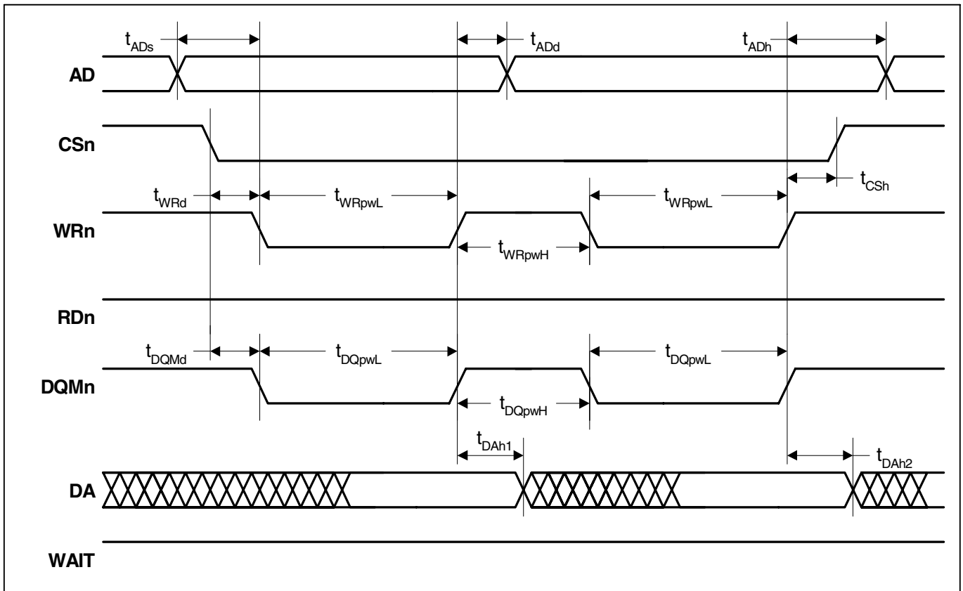
Figure 9. Static Memory Multiple Word Write 16 bit Cycle Timing Measurement
