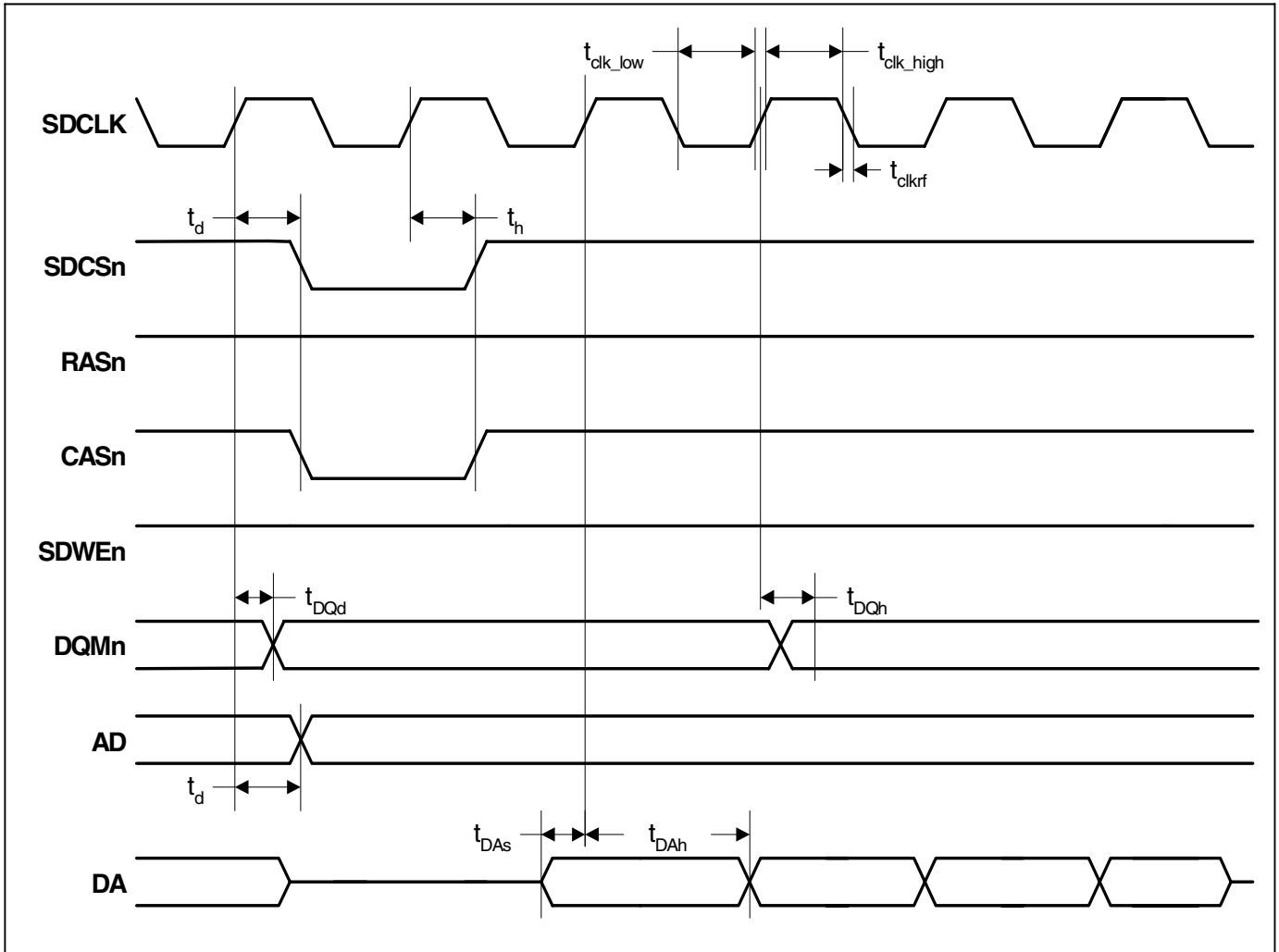
Figure 3. SDRAM Burst Read Cycle Timing Measurement
