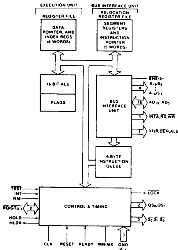
Figure 1. 8086 CPU Block Diagram
