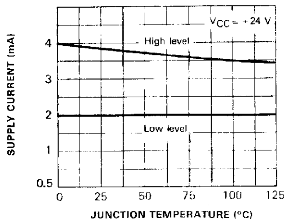
Figure 7: Supply Current vs. Junction Temperature
