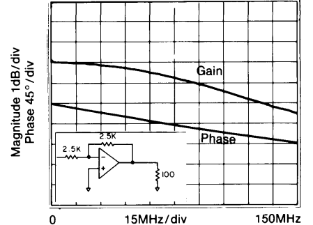
Frequency Response, A_V = -1 , R_f = 2.5k\Omega
