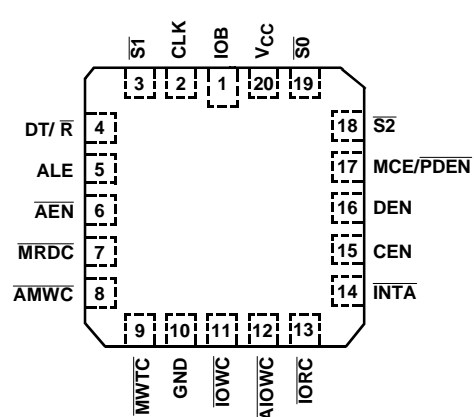
20 LEAD PLCC, CLCC TOP VIEW
