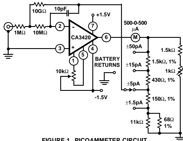
FIGURE 1. PICOAMMETER CIRCUIT
