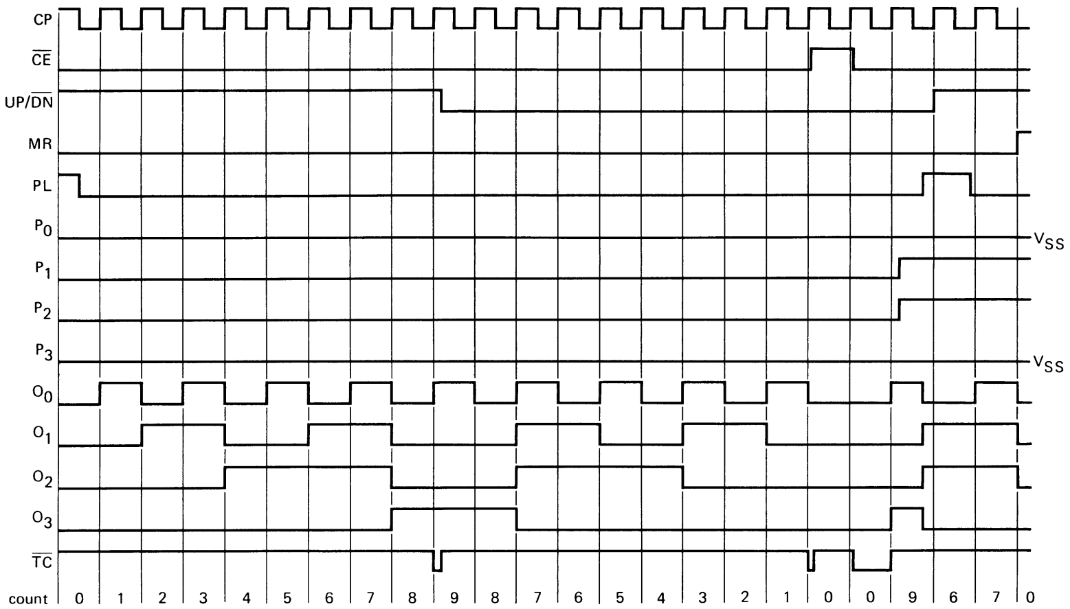
Fig.8 Timing diagram.
