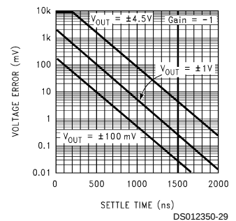
Voltage Error vs. Settle Time
