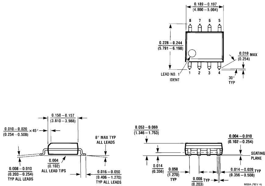
8-Lead (0.150") Molded Small Outline Package, JEDEC Ordering Number LM6152ACM or LM6152BCM NSC Package Number M08A
