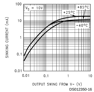
Output Voltage vs. Sink Current
