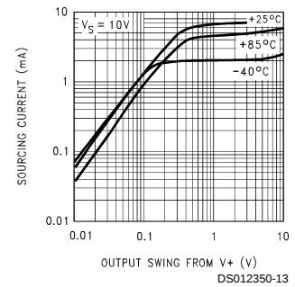
Output Voltage vs. Source Current
