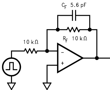
FIGURE 1. Typical Inverting Gain Circuit A_V = -1
