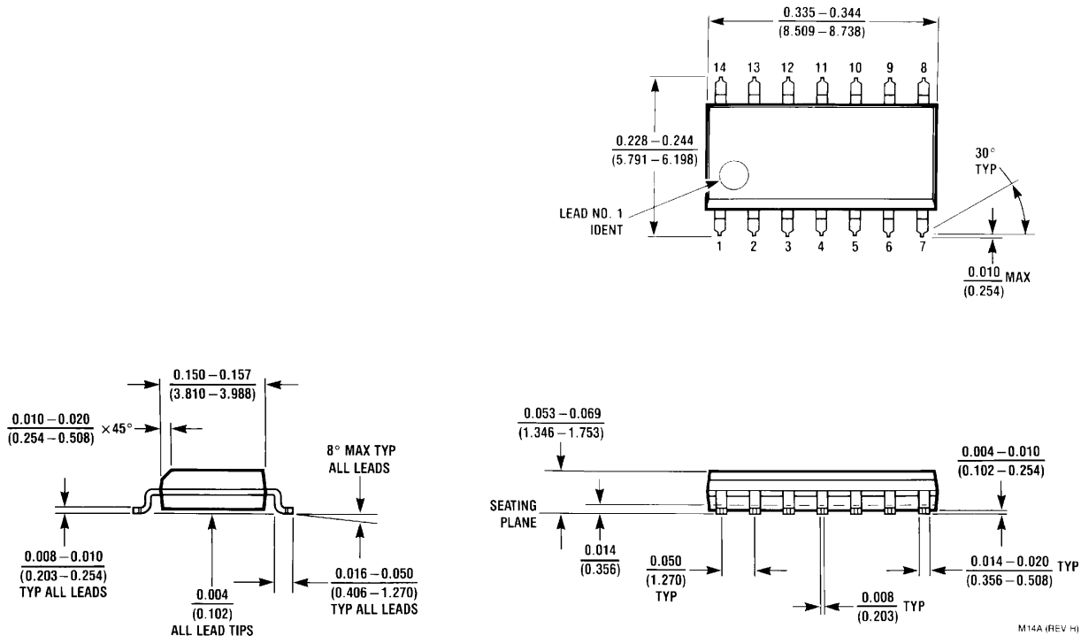
14-Lead (0.150") Molded Small Outline Package, JEDEC Order Number LM6154BCM NSC Package Number M14A
