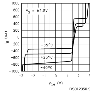
Bias Current vs. V_{CM}
