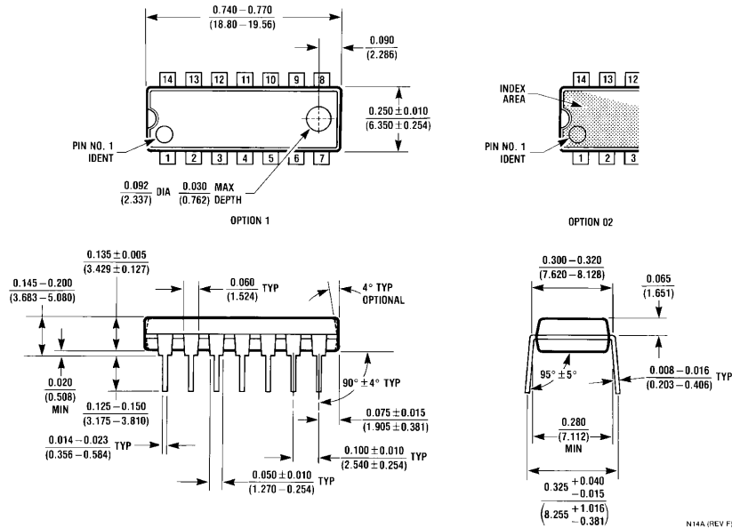
14-Lead (0.300" Wide) Molded Dual-In-Line Package, JEDEC Order Number LM6154ACN or LM6154BCN NSC Package Number N14A
