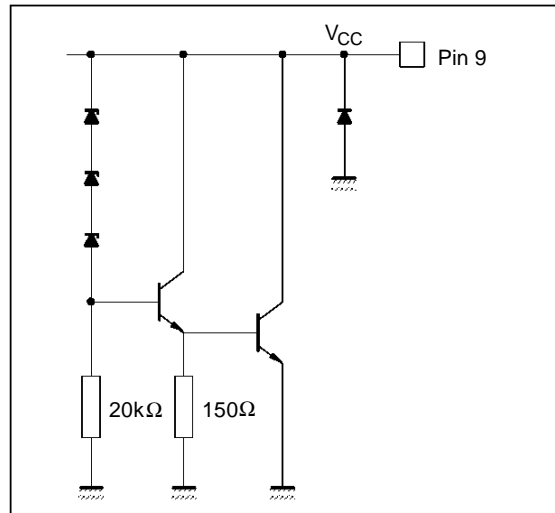
Figure 4 : V CC Pin Configuration
