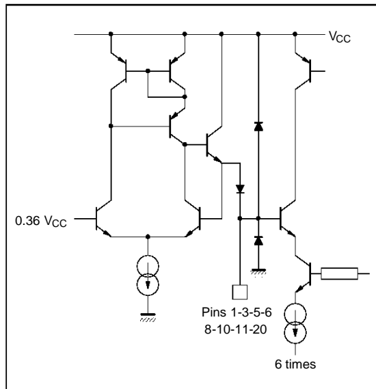
Figure 1 : Input Configuration
