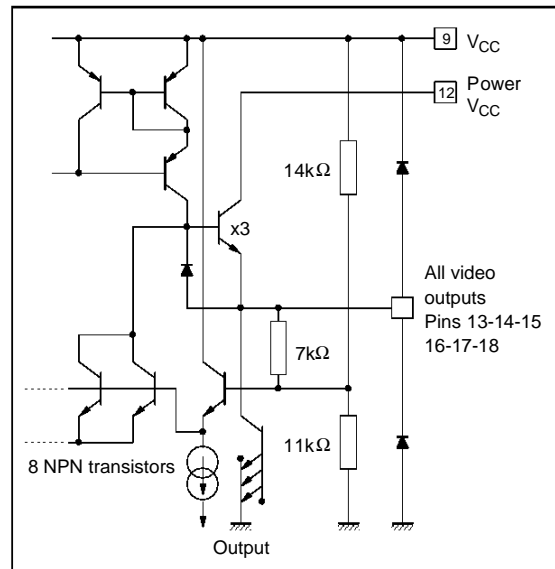
Figure 2 : Output Configuration
