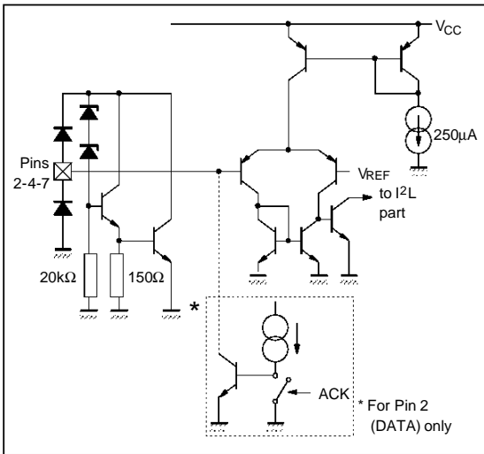
Figure 3 : Bus I/O Configuration
