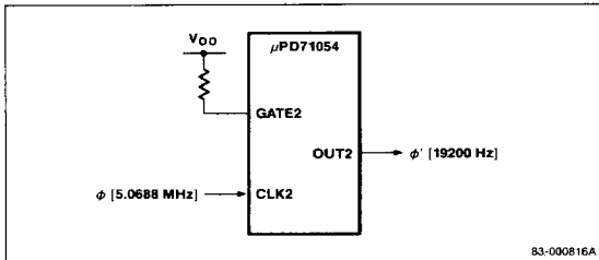
Figure 15. Frequency Division
