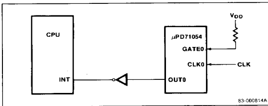
Figure 13. Mode 2 Configuration
