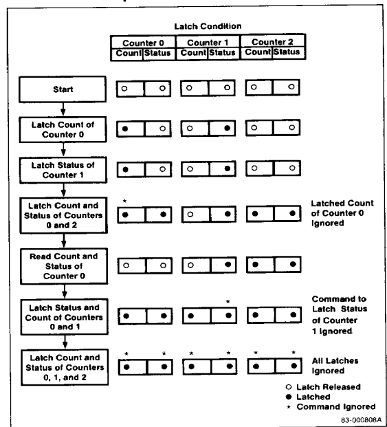
Figure 7. Multiple Latch Command Execution Example
