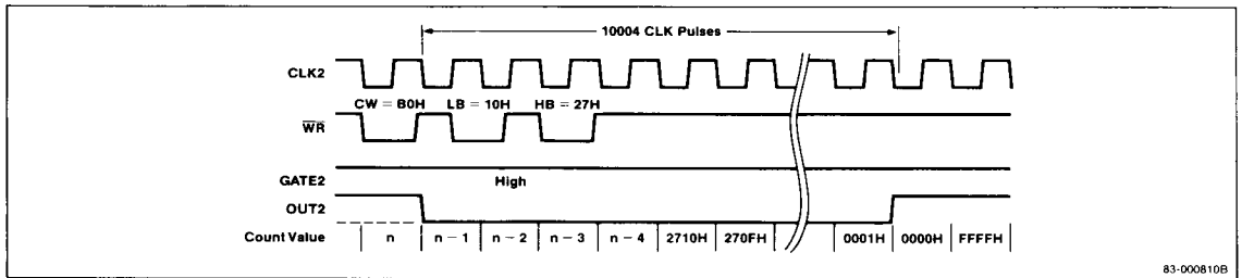
Figure 9. Mode 0 Program Example Timing Chart
