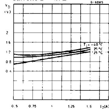
Figure 17. Dropout voltage between pin 7 and pin 2 vs. current at pin 2
