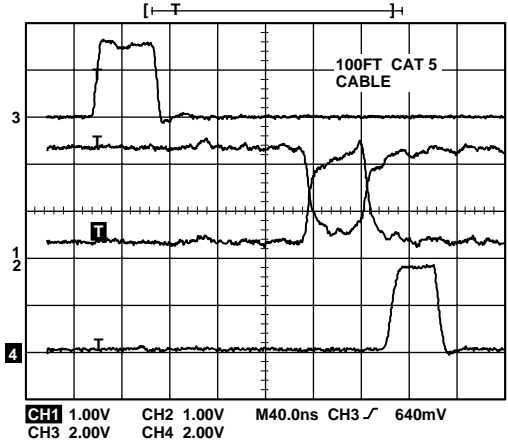
Figure 21. Driving 100 ft. Cable H-L Transition
