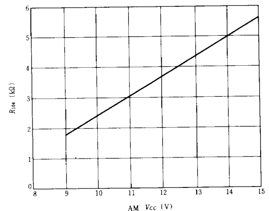
■ R 104 (Resistor of Pin-15) vs. AM V cc
