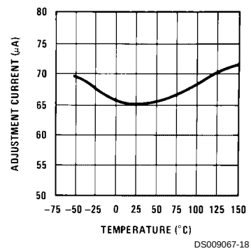
Adjustment Current
