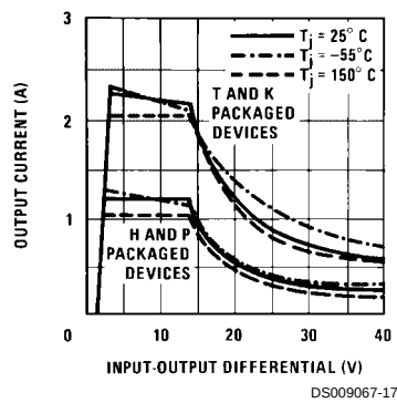
Current Limit
