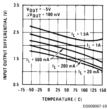
Dropout Voltage
