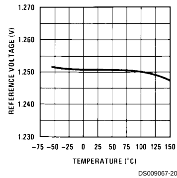
Temperature Stability
