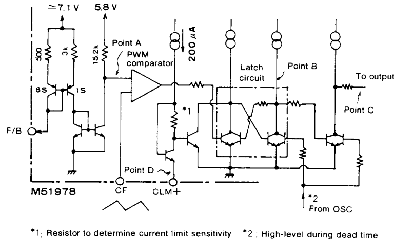
Fig.9 PWM comparator section, PWM latch and current limit latch section
