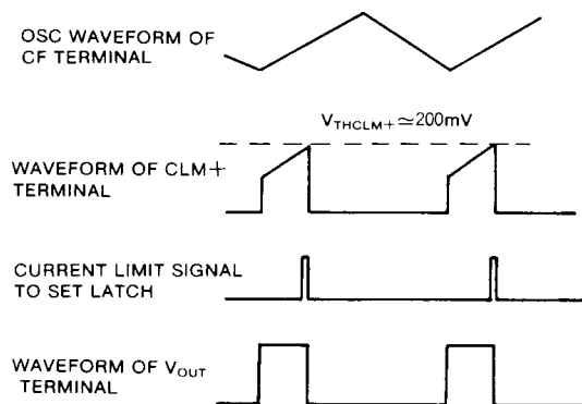
Fig.11 Operating waveforms of current limiting circuit
