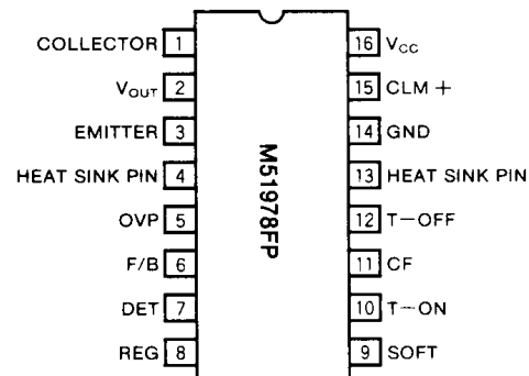
Outline 16P2N
