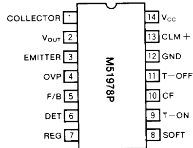
Outline 14P4
