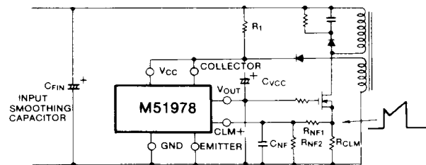
Fig. 24 Peripheral circuit diagram of CLM + terminal
