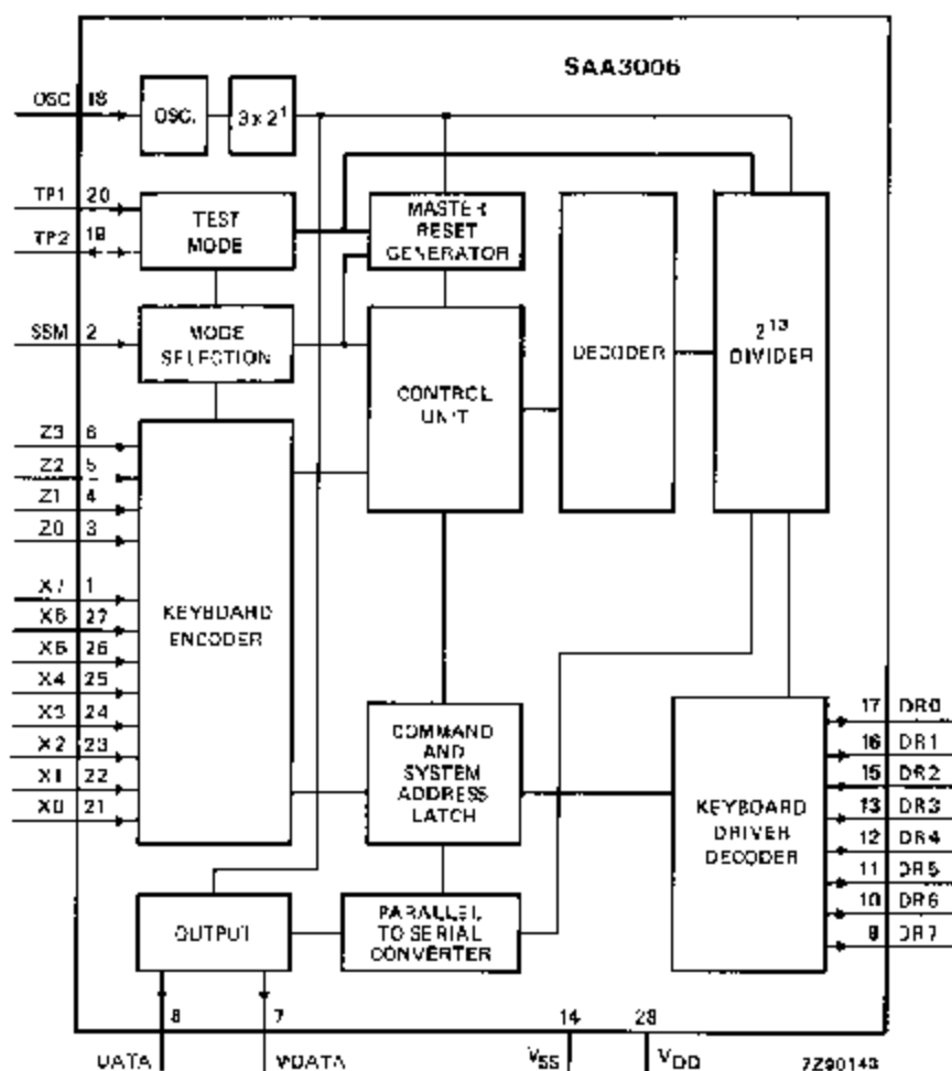
Fig. 1 Block diagram.
