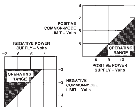
Figure 16. Common-Mode Range vs. Power Supply
