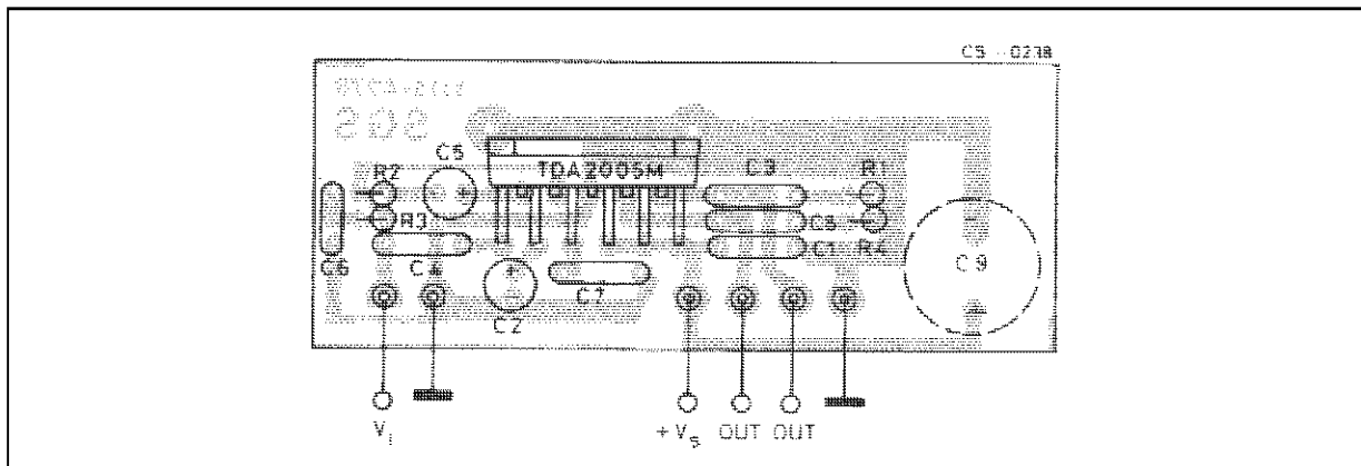
Figure 28 : P.C. Board and Components Layout of Figure 27 (1:1 scale)
