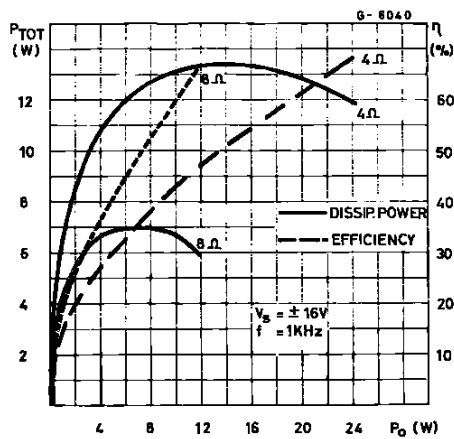
Figure 9 : Power Dissipation versus Output Power
