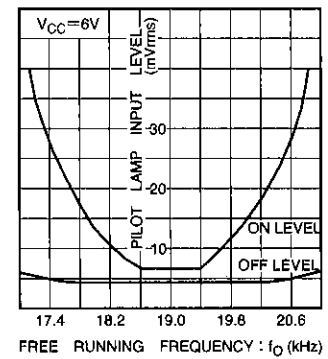
Fig. 7 Lamp on and off levels vs. free-running frequency
