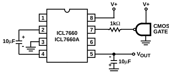
FIGURE 17. EXTERNAL CLOCKING
