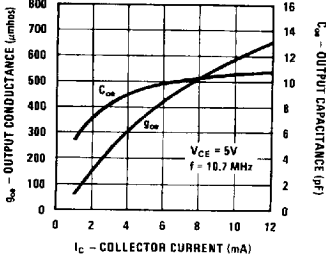
g oe and C oe vs Collector Current
