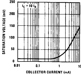
Saturation Voltage vs Collector Current
