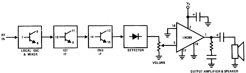
FIGURE 1. AM Radio
