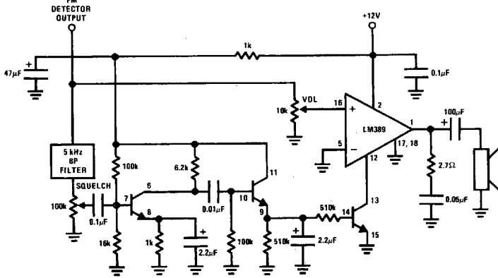
FIGURE 4. FM Scanner Noise Squelch Circuit
