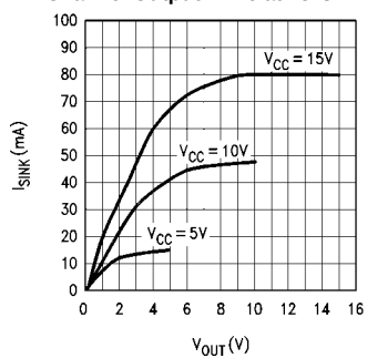
N-Channel Output Drive at 25^\circ\text{C}
