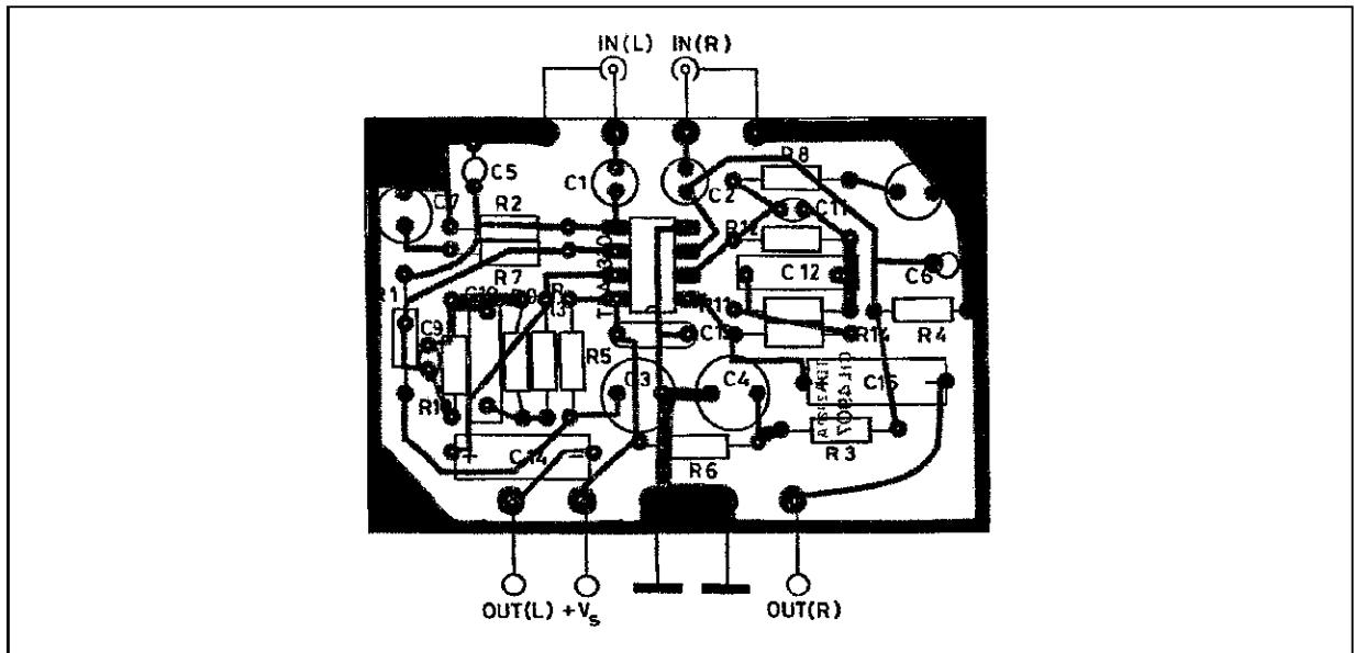
Figure 13 :P.C. Board and Components layout of the Circuit of figure 12
