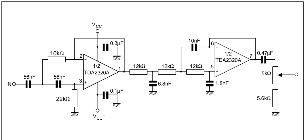
Figure 19 : Subsonic Filter
