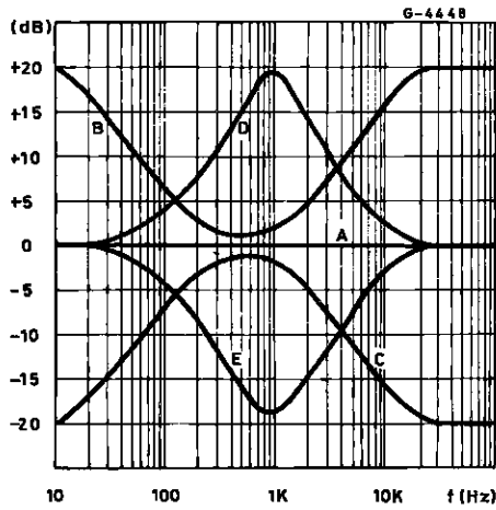
Figure 24 : Frequency Response of the Circuit of figure 23
