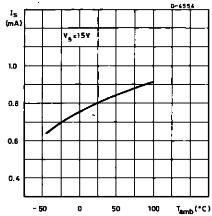
Figure 4 : Supply Current versus Ambient Temperature
