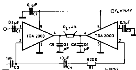
Figure 20. Low cost bridge configuration application circuit (*) ( P_0 = 18W )
