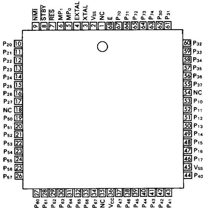
(Top View)
