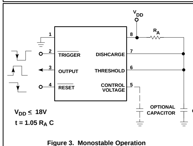
Figure 3. Monostable Operation
