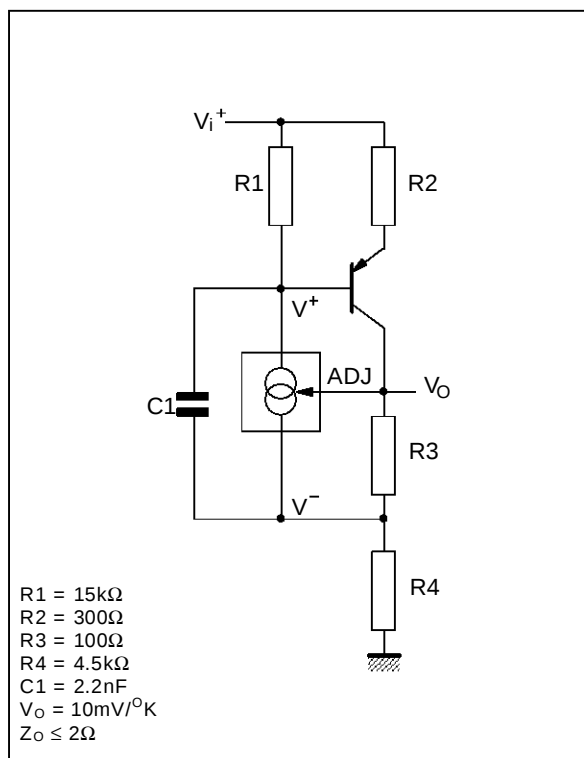
Figure 8 : Low Input Voltage Reference Driver
