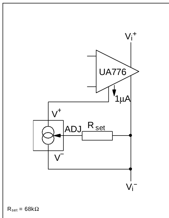
Figure 7 : Micropower Bias
