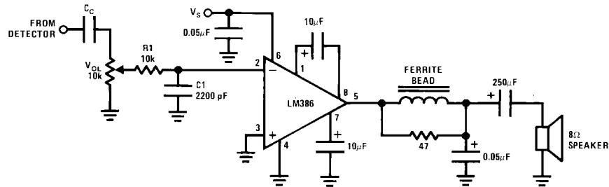
AM Radio Power Amplifier
