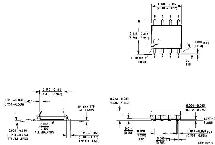
SO Package (M) Order Number LM386M-1 NS Package Number M08A
