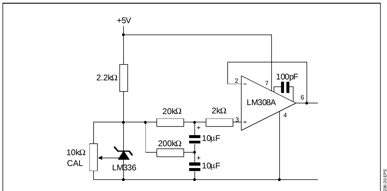
Figure 10 : Low Noise Buffered Reference
