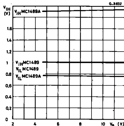
Figure 11 : Input Threshold versus Power Supply Voltage
