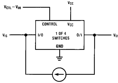
FIGURE 1. "ON" Resistance
