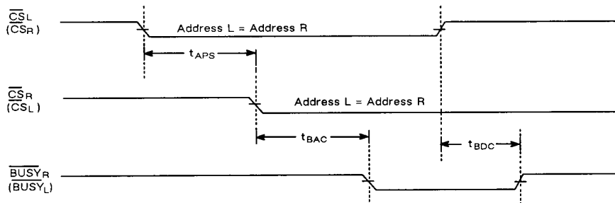
Data Contention Cycle No. 2 ( \overline{CS} Controlled) 1, 3 :
