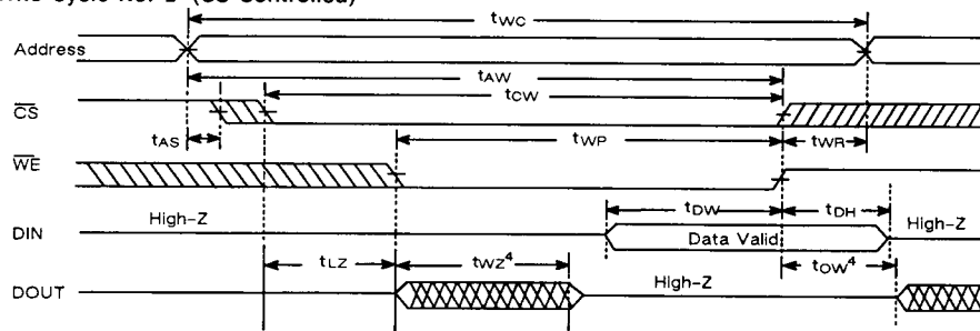
Write Cycle No. 2 ( \overline{CS} Controlled) 1,2,3
