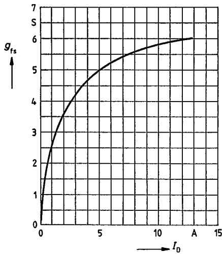
Typical transconductance
