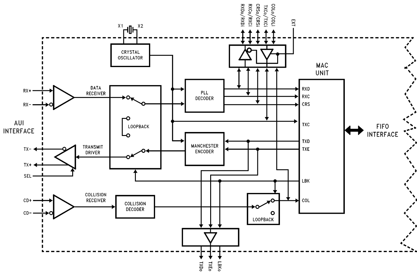
FIGURE 1-2. Block Diagram of Ethernet ENDEC
