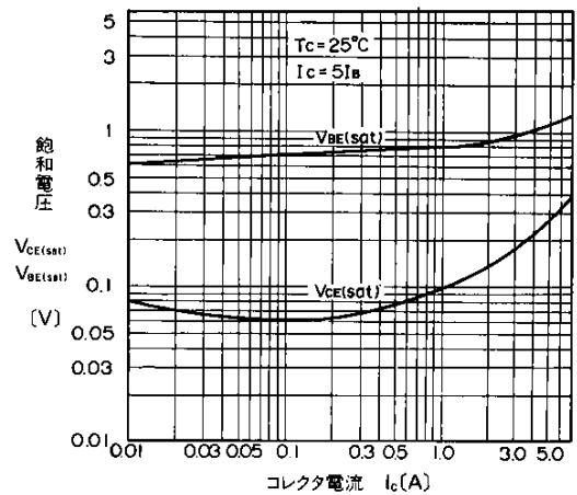
Base and Collector Saturation Voltage
