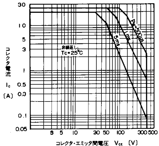
Soft Operating Area
