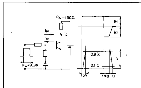
Switching Time
